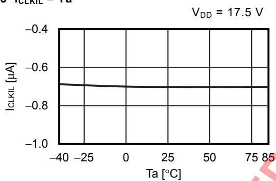
5.3 I_{CLKIL} - T_a
