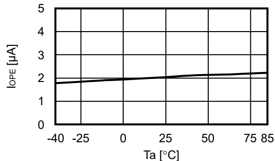
1.2 I OPe – Ta
