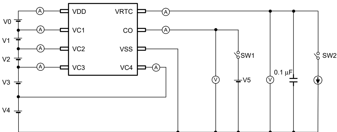
Figure 4 Test Circuit 2
