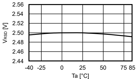
2. 3 V_{RSD} vs. T_a
