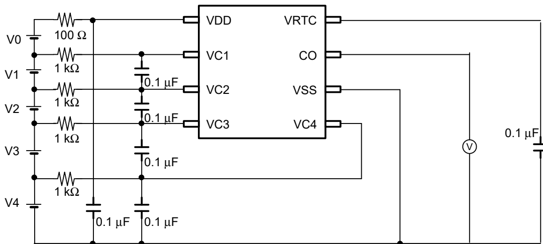
Figure 3 Test Circuit 1
