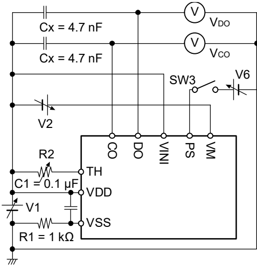
Figure 5 Test Circuit 1
