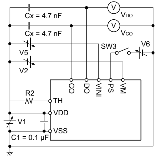
Figure 6 Test Circuit 2
