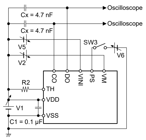
Figure 10 Test Circuit 6
