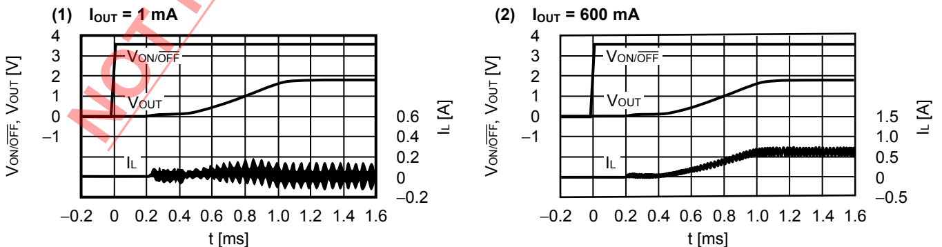
3.2 ON/OFF 端子响应 ( V_{OUT} = 1.8V , V_{IN} = 3.6V , V_{ON/OFF} = 0V \rightarrow 3.6V , T_a = +25^\circ C )
