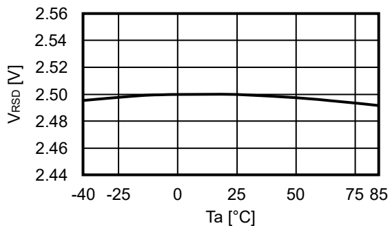
2.3 V_{RSD} - T_a
