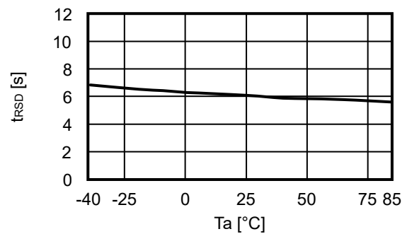
3.2 t_{rSD} - T_a
