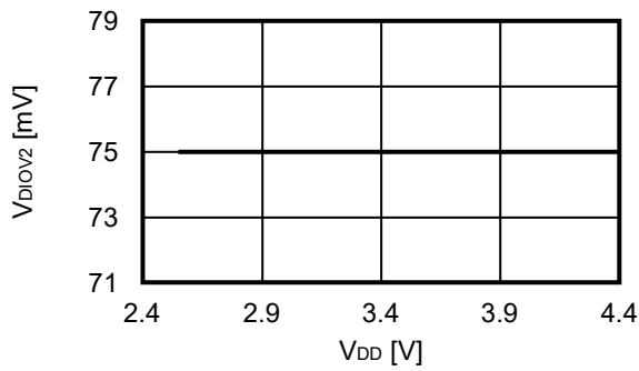
2.7 V_{DIOV2} - V_{DD}
